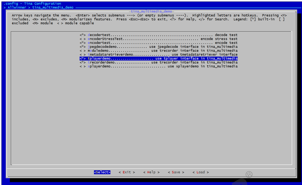
图 2-7: tplayerdemoConfig
