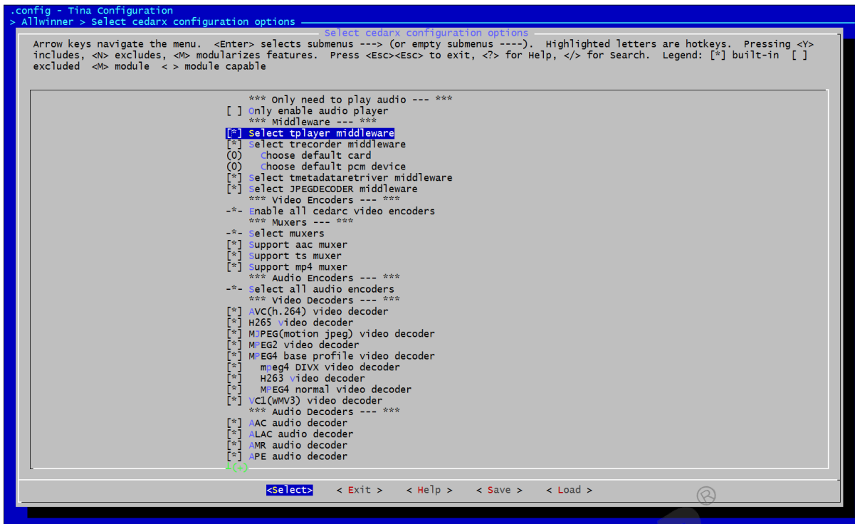
图 2-6: tplayerConfig
